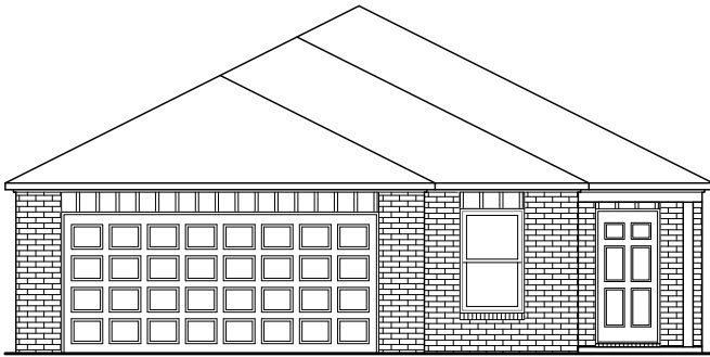
RC Armstrong II Elevation C
