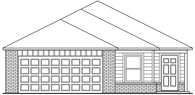
RC Armstrong II Elevation B
